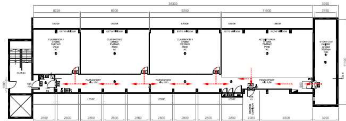
FIRE ESCAPE ROUTE FOR UNIT #05-01 (2-WAY EXIT) SCALE: 1: 100
