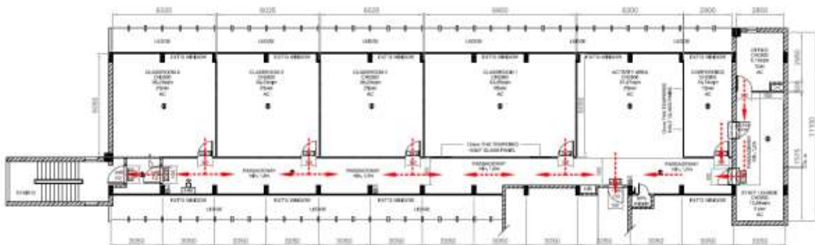
FIRE ESCAPE ROUTE FOR UNIT #05-02 (2-WAY EXIT) SCALE: NTS
